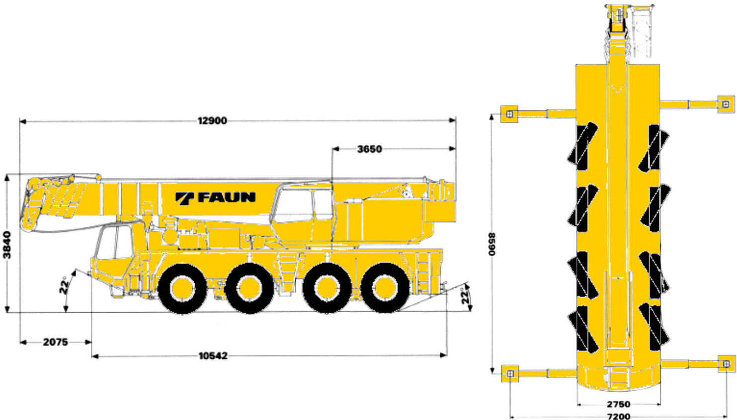
Faun ATF 90-4
